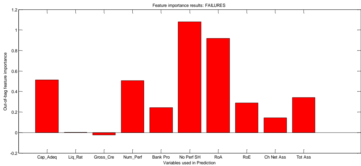
Figure 6: Decision Trees Model using Two-year Sample showing variable importance for bank FAILURE & SURVIVAL prediction
