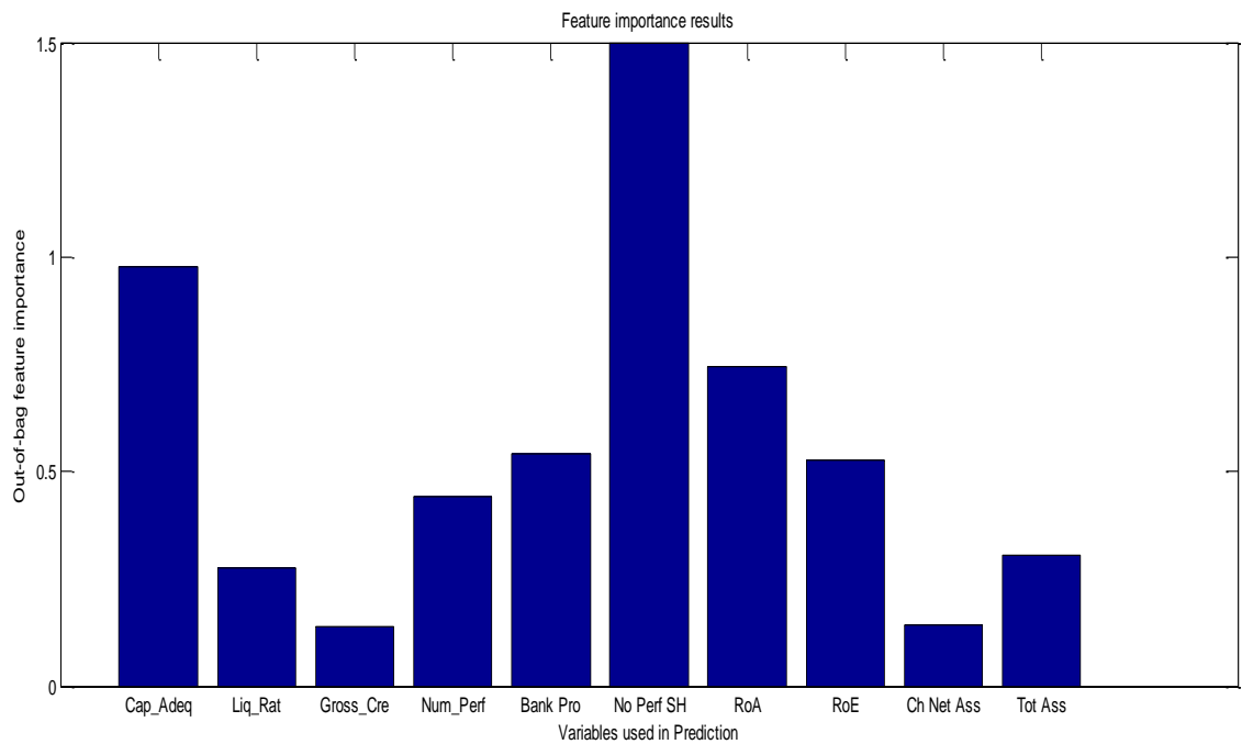
Figure 1: Decision Trees Full Sample factor importance for distress prediction
