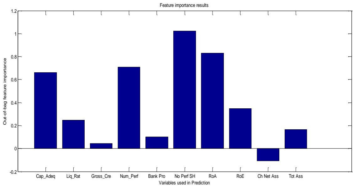
Figure 2: Decision Trees One-year Sample variable importance for distress prediction
